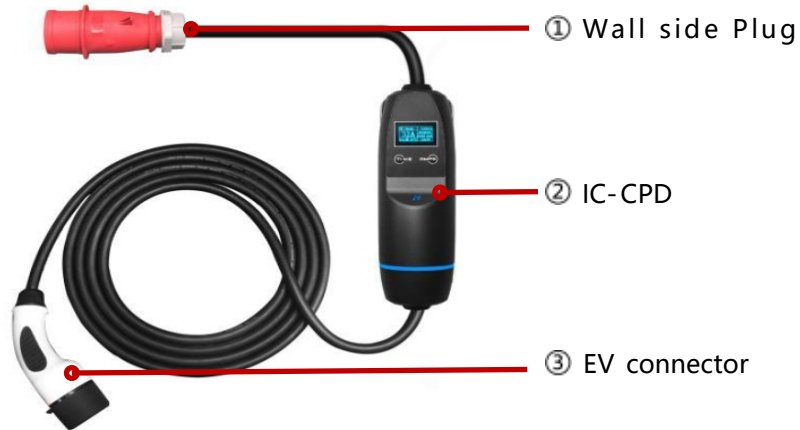
Figure 1 Schematic
