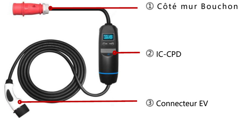
Figure 1 Schéma
